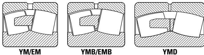
Fig. 4. Machined cages.
