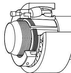
Fig. 28. Hydraulic nut used to withdraw a push-type adapter sleeve.
