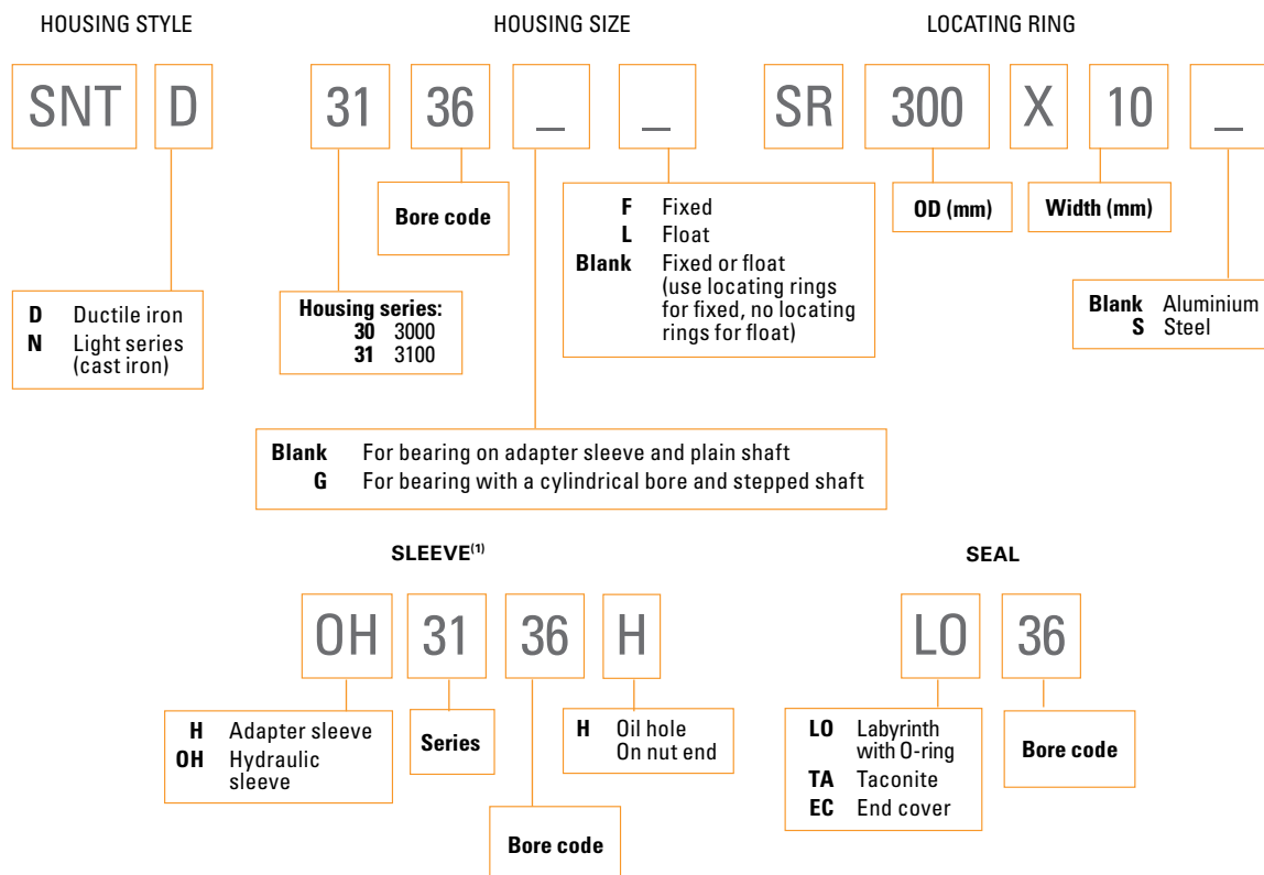
Fig. 7. SNT nomenclature: 3000 and 3100 series.
