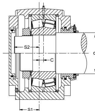
Fig. 14. Cylindrical bore bearing end cover/taconite seal.
