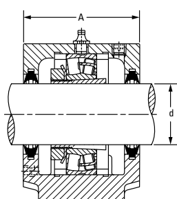
Double-Lip Seal
