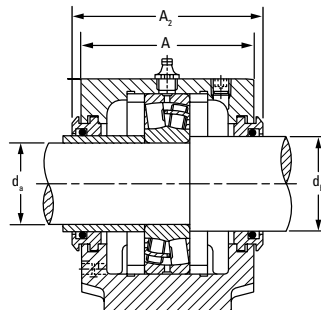
Labyrinth Seal
