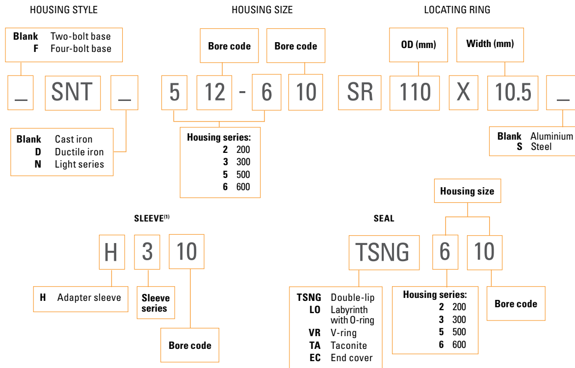
Fig. 6. SNT nomenclature: 200-300 and 500-600 series.
