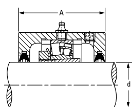
Double-Lip Seal
