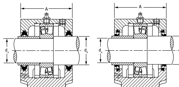
Double-Lip Seal
