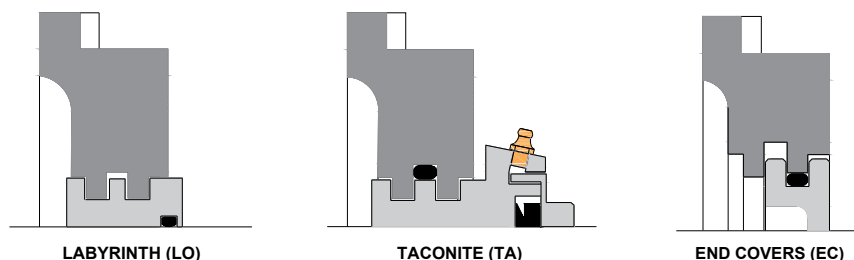
Fig. 3. Seal options: 3000 and 3100 series.
