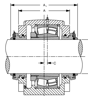
Taconite Seal
