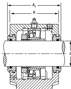
Labyrinth Seal
