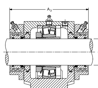
Taconite Seal
