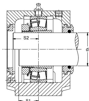
Fig. 11. Tapered bore bearing on adapter sleeve end cover/labyrinth seal.
