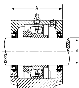
V-Ring Seal
