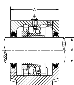
Double-Lip Seal
