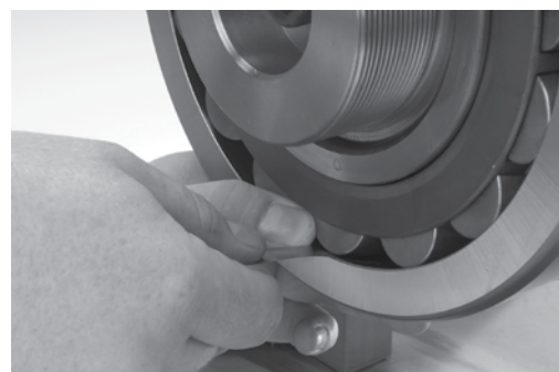
Fig. 10. After mounting, the RIC should be checked at the unloaded roller.
