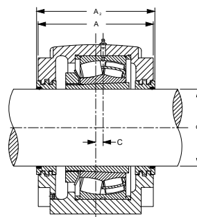
Labyrinth Seal
