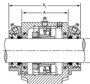
Taconite Seal
