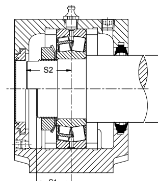
Fig. 12. Cylindrical bore bearing end cover/double-lip seal.
