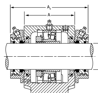
Taconite Seal
