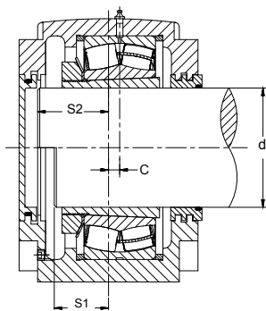
Fig. 13. Tapered bore bearing on adapter sleeve end cover/labyrinth seal.
