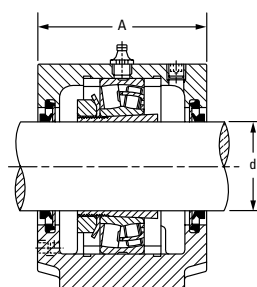
V-Ring Seal
