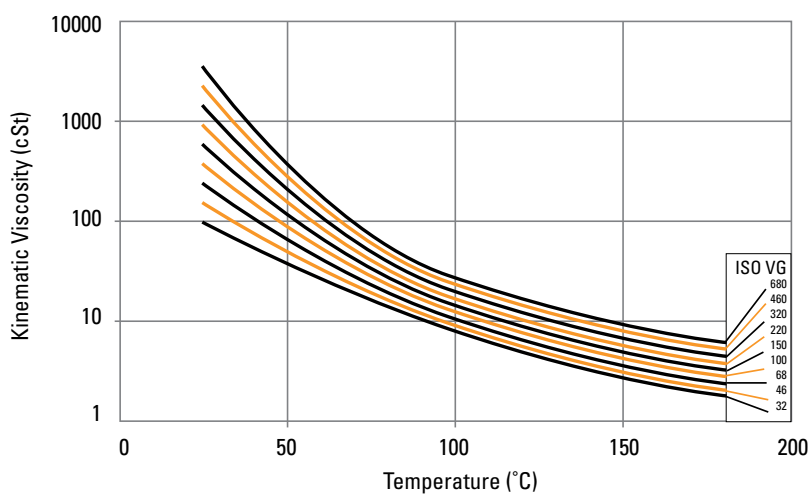
Fig. 73. Temperature vs. kinematic viscosity.
