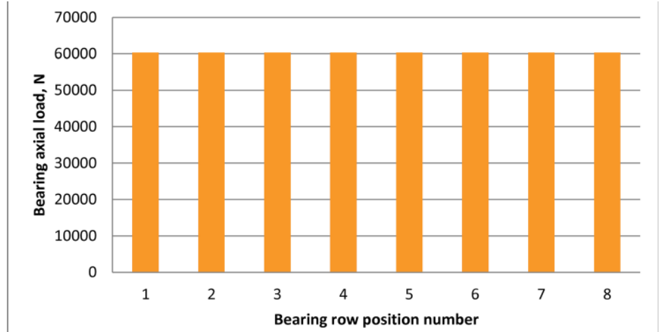
Figure 5 shows the calculated bearing axial loads in each row, when optimizing the spacer stiffness ratio.
