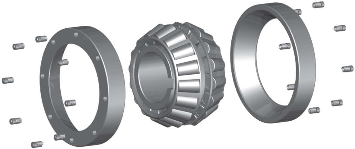
Fig. 53. TDIK bearing.
