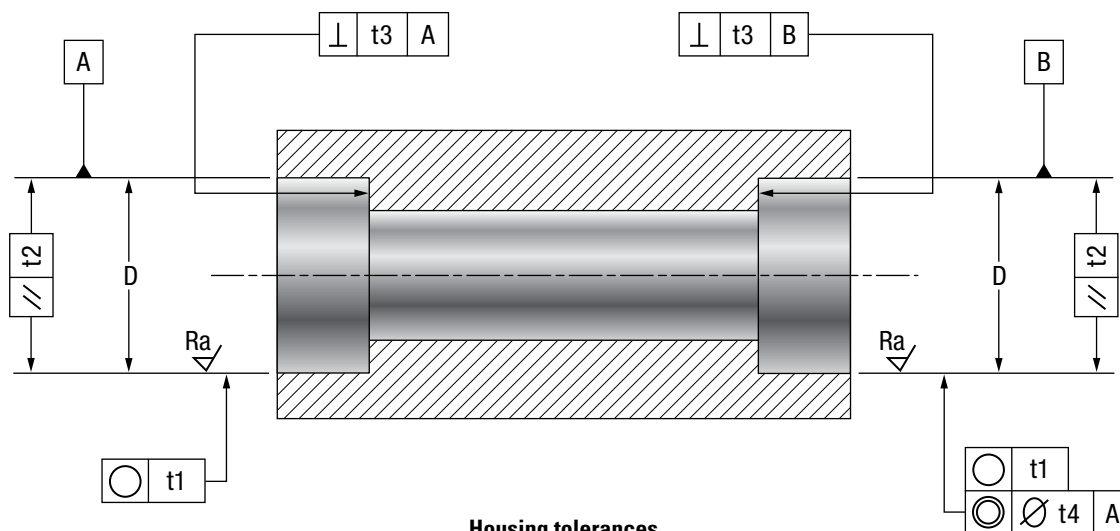
Housing tolerances
